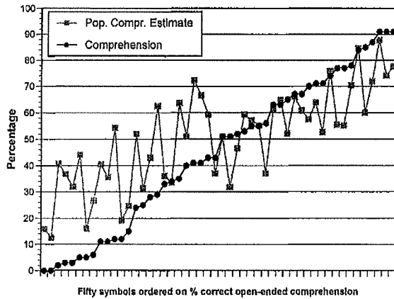
Figure 1: Plot of comprehension and predicted population comprehension estimates
